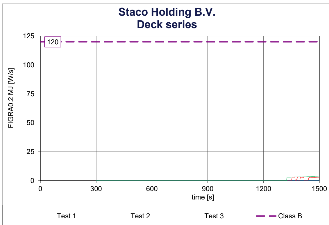
Chart 5: FIGRA 0.2 MJ [W/s]
